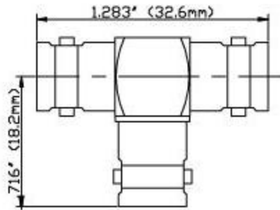
Title: BNC Female T Adapter
